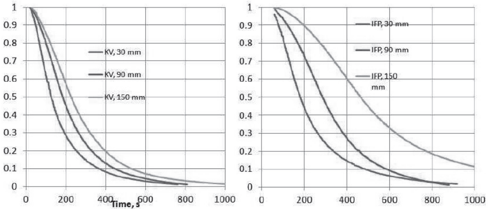
Figure 6 The drainage, z vs. time (s) for KV, AFF and IFP, AFFF foams
