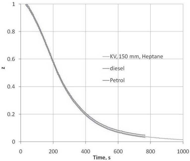
Figure 9 Drained fraction vs time, for KV AFFF foam with heptane, petrol and diesel liquid-foam interfaces.
