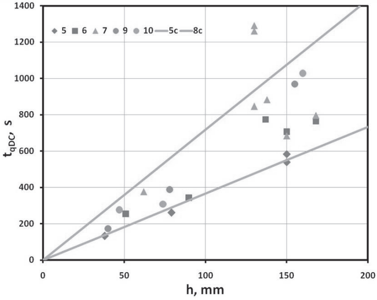
Figure 8 The quarter drain time (s) corrected for expansion ratio with foam height (mm) for the foams KVAFFF-3-6 (5), FEAFFF-1-3 (6), FEAFFF-1-5 (7), KVARAFFF-3-5 (8), IFPAFFF-3-5 (9), and IFPAFFF-3-6 (10) along with correlation lines for KVAFFF-3-6 (5c) and KVARAFFF-3-5 (8c)
