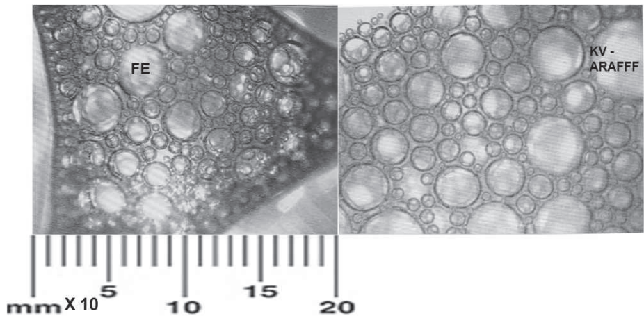
Figure 5 Foam bubbles under a microscope - FE and KV AR-AFFF
