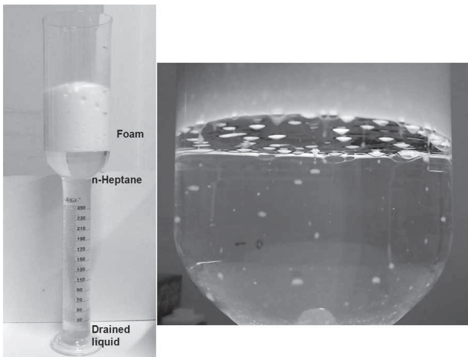
Figure 1 The foam drainage apparatus (left) and the drainage process (right)
