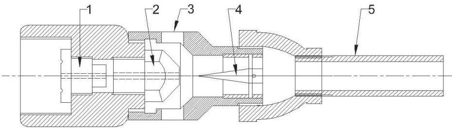
Figure 3 Foam nozzle used to generate the foam
