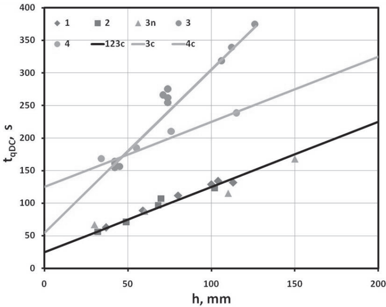
Figure 7 The quarter drain time (s) corrected for expansion ratio with foam height (mm) for the foams KVAFFF-3-3 (1), FEAFF-1-1 (2), IFPAFFF-3-3 (produced using a nozzle, 3n) along with correlation named 123c, IFP-3-3 (3) and KVARAFF-3-3 (4)
